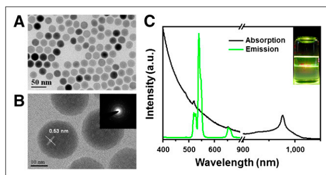
FIGURE 2. (A) TEM bright-field image. (B) High-resolution TEM image of NaGdF 4 :Yb 3+ /Er 3+ and selected area electron diffraction pattern (inset). (C) Emission spectra (green) and ultraviolet-visible spectra (black) of NaGdF 4 :Yb 3+ /Er 3+ and upconversion luminescence of UCNP in toluene under excitation of 980-nm laser (inset). a.u. = arbitrary units.
