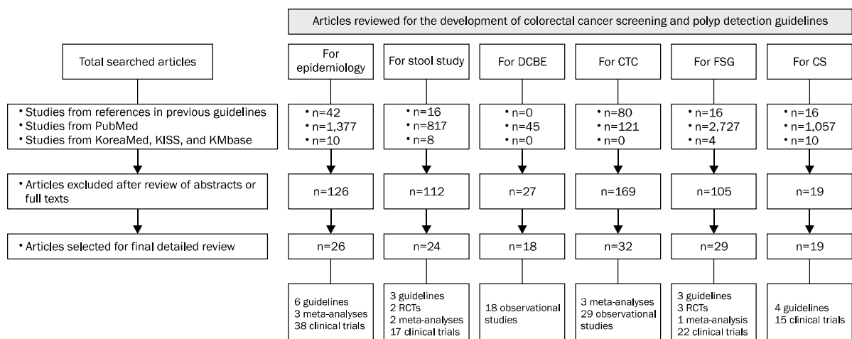
Fig. 1. Study selection.
