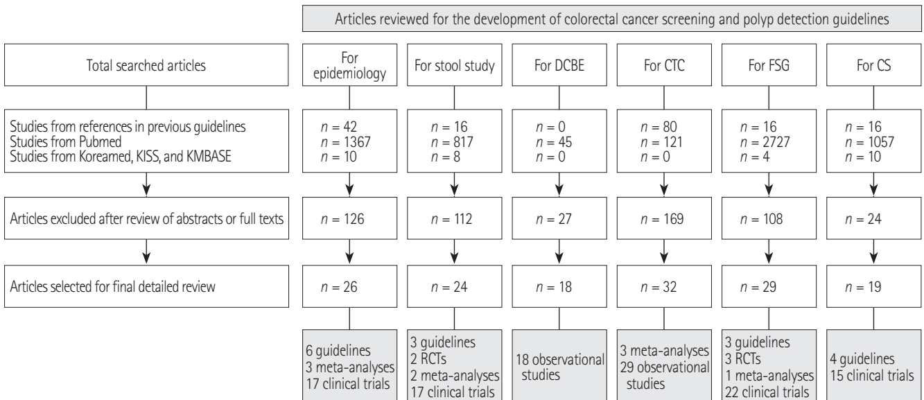
Fig. 1. Study selection.
