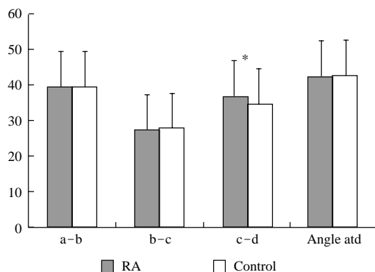
Fig. 5. Palmprint ridges a-b, b-c, c-d and palmprint angle atd (unit: degree) in the rheumatoid arthritis (RA) (89 persons) and the control (1,178 persons), *: P<0.05
