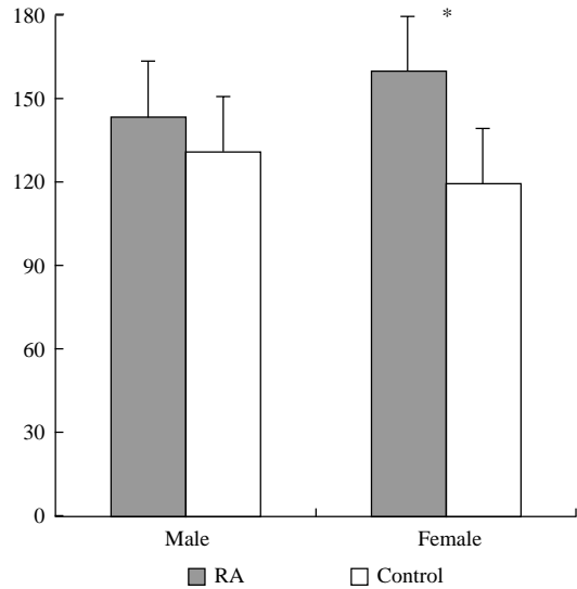
Fig. 2. Total fingerprint ridges in the rheumatoid arthritis (RA) (41 cases) and the control (557 cases), Between the RA and the control, *: P < 0.05
