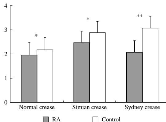
Fig. 6. Total degree of palm crease transversality in the rheumatoid arthritis (RA) (58 persons) and the control (5,176 persons), *: P<0.05, **: P<0.01
