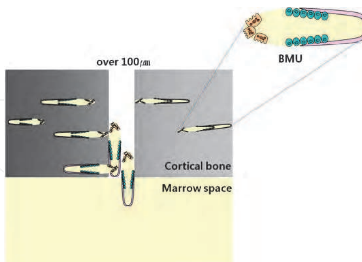
Fig. 9. Schematic diagram of the gap healing.
