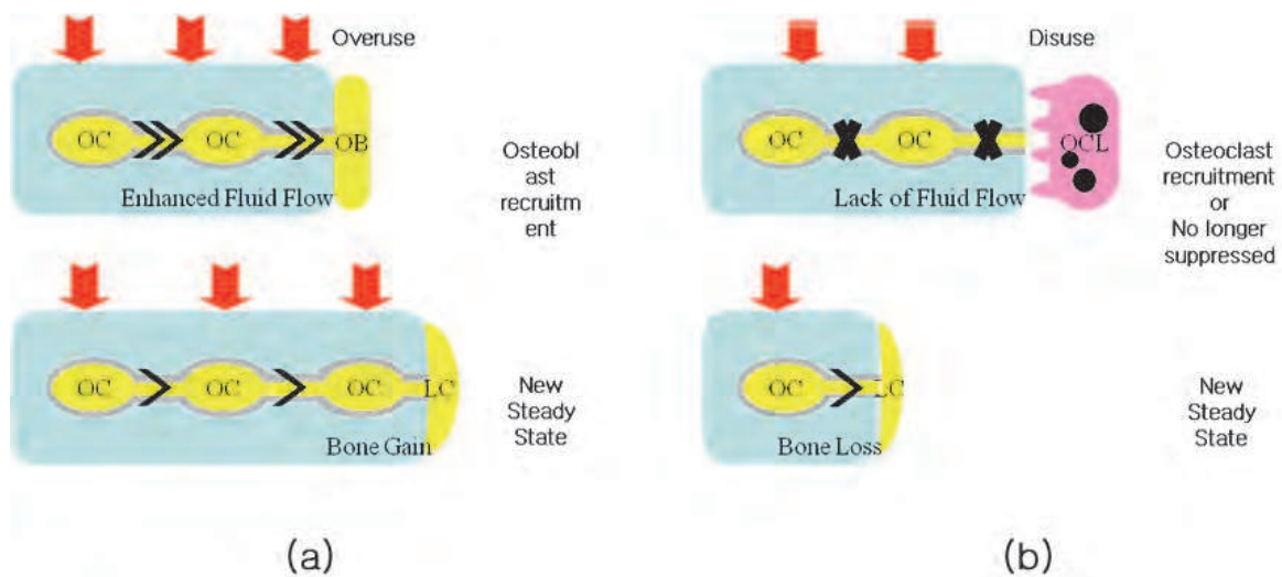
Fig. 3. Schematic diagram of mechanotransduction.
