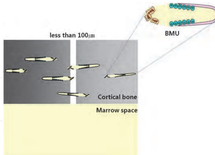
Fig. 8. Schematic diagram of the contact healing.
