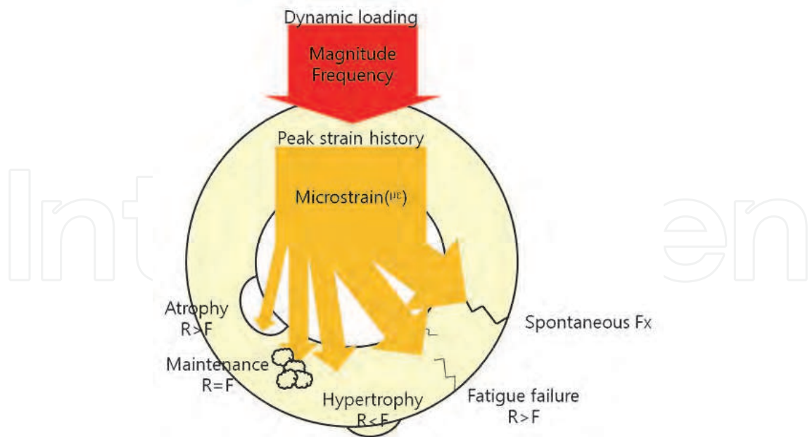
Fig. 2. The concept of the mechanostat.
