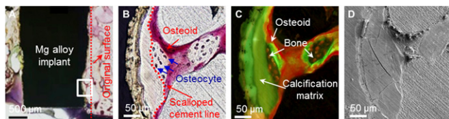
Fig. 1. Histological and SEM analysis of rabbit femoral condyle after 8 wk of implantation of \varnothing 2 \times 6 -mm cylindrical Mg alloy implant. (A) Implant–bone interface at low magnification, the degradation of the Mg alloy implant is evidenced by drawing the original surface line. Magnified image of bone formation region observed by (B) light microscopy, (C) fluorescence microscopy, and (D) SEM.
